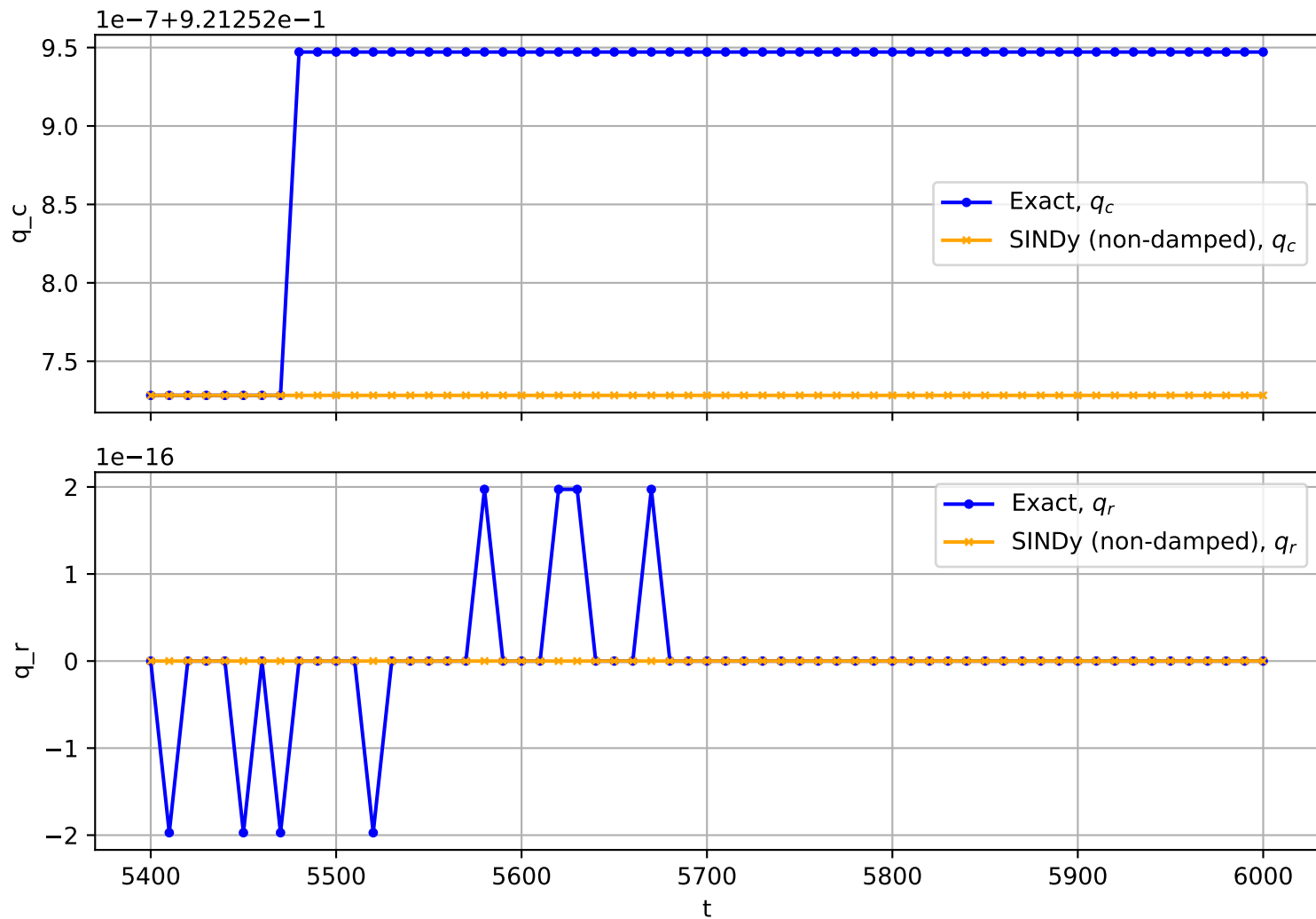
Trajectory No. 1588
