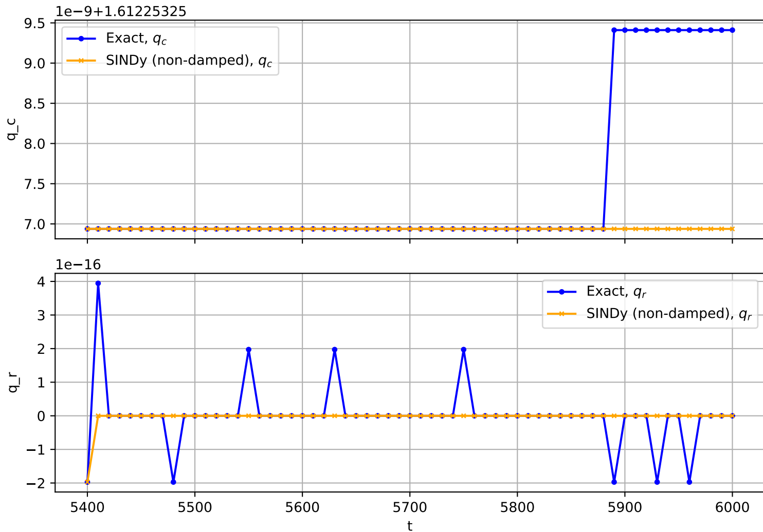
Trajectory No. 1593
