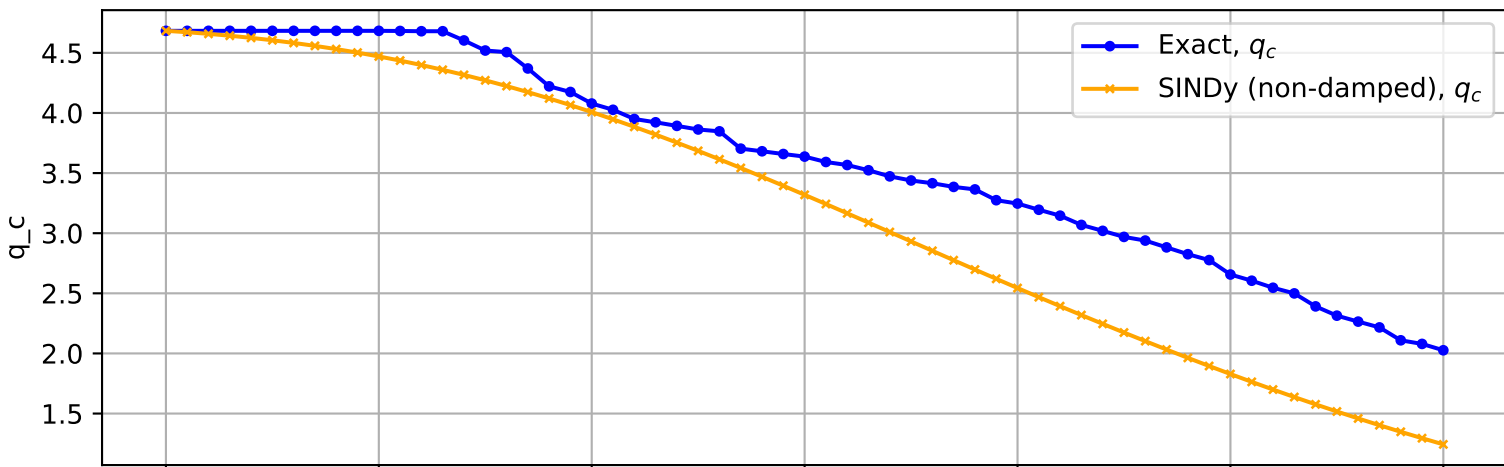
Trajectory No. 1602
