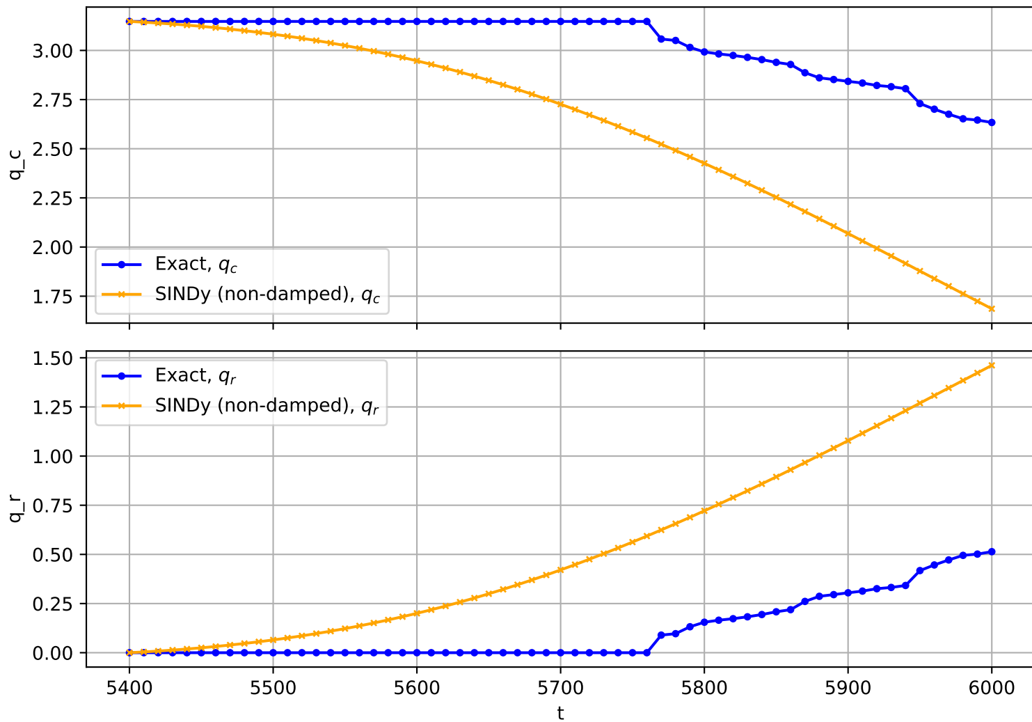
Trajectory No. 1605
