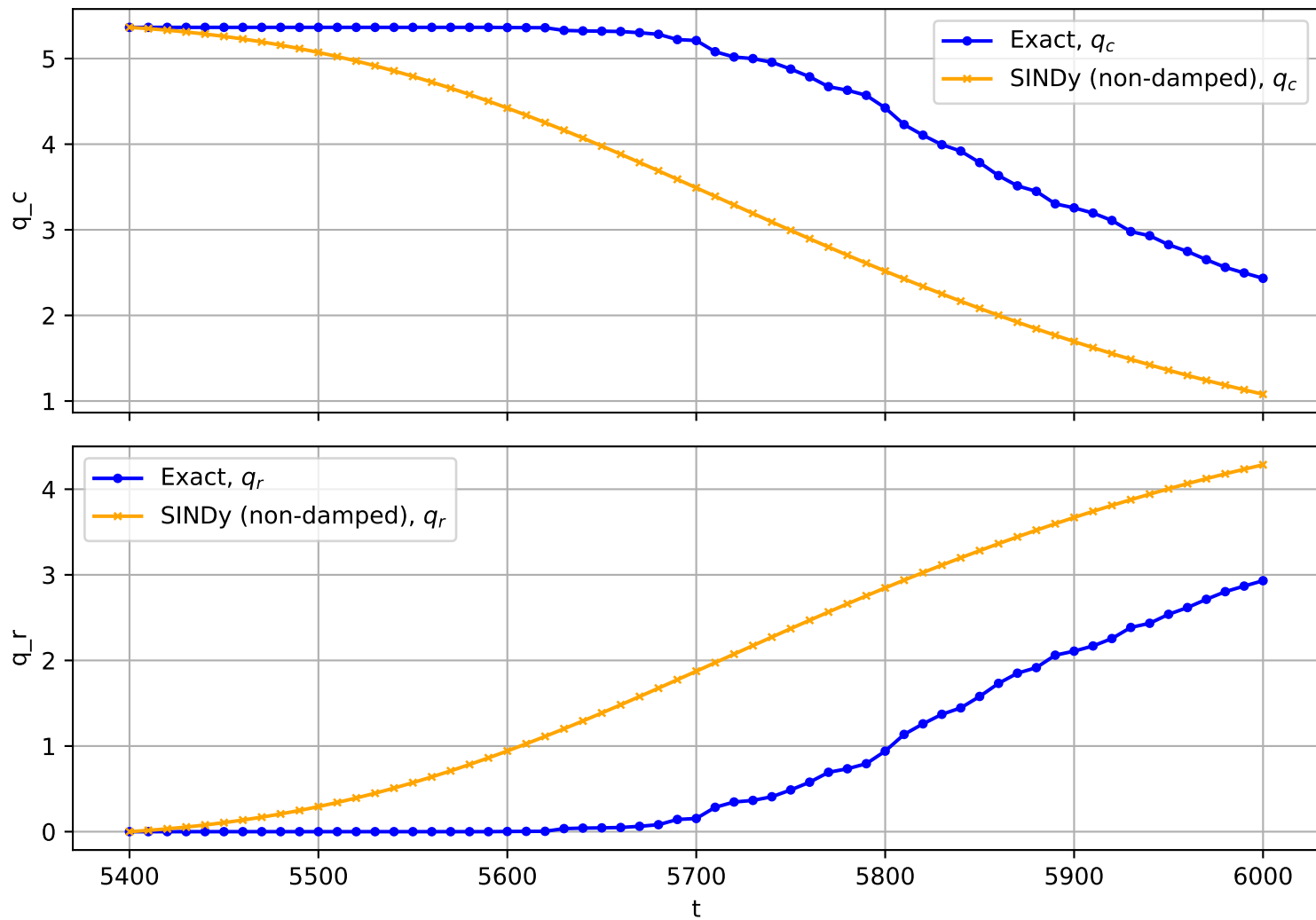
Trajectory No. 1626
