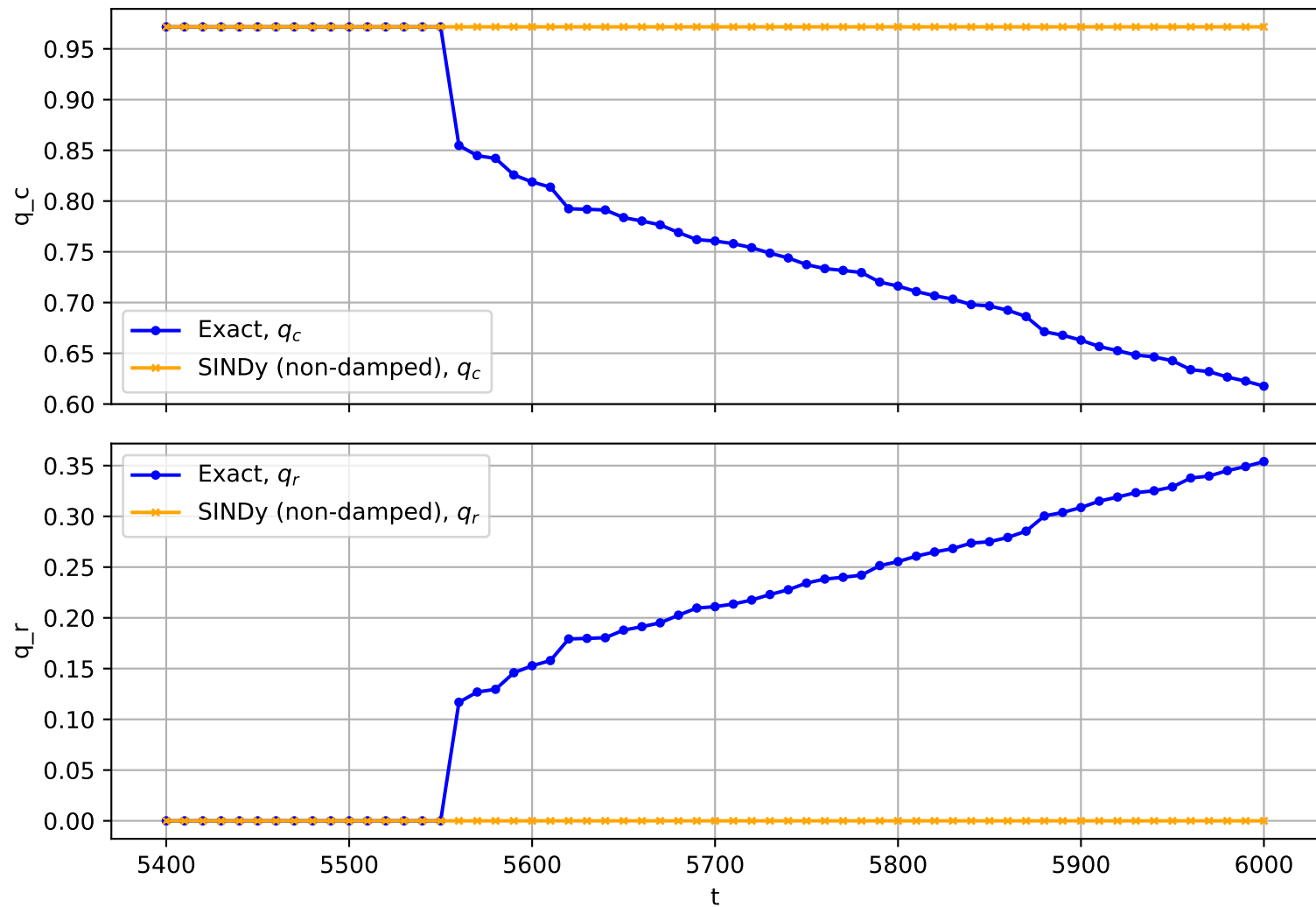
Trajectory No. 164
