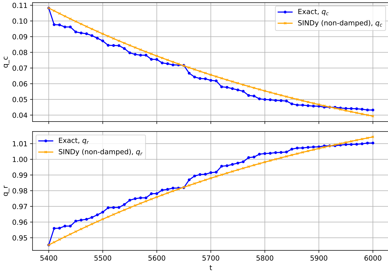
Trajectory No. 1671
