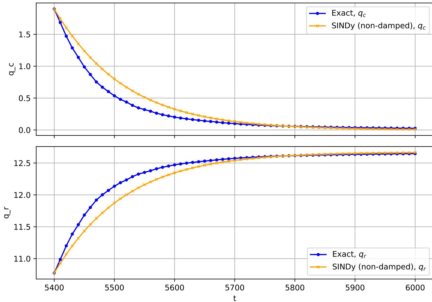
Trajectory No. 1696
