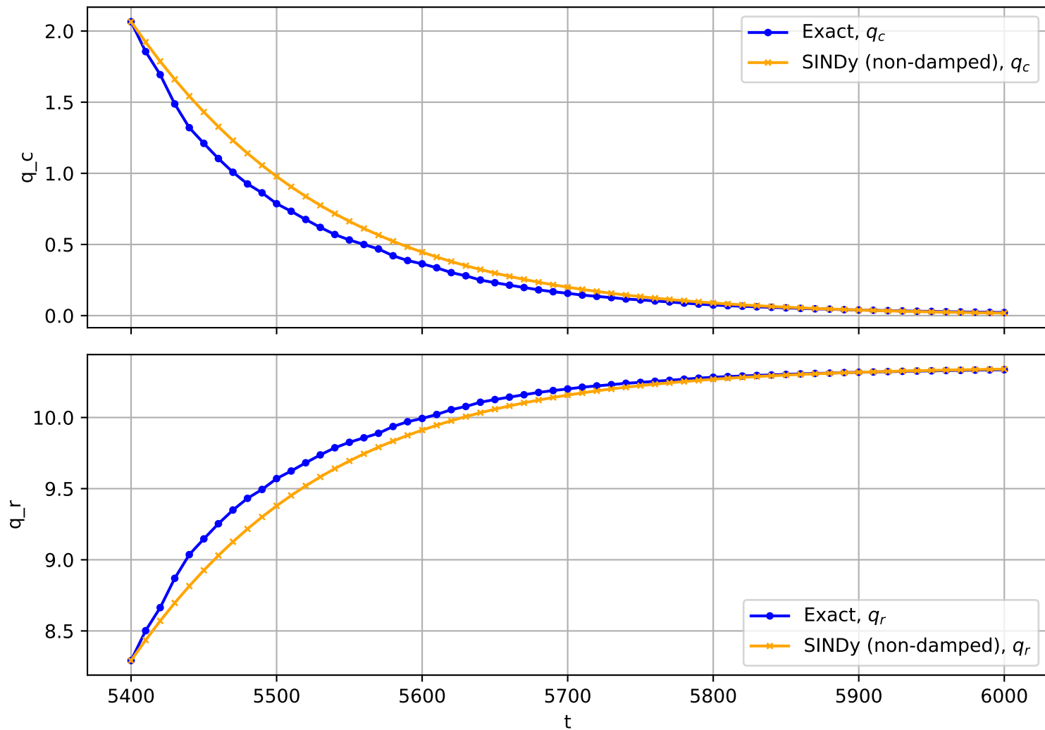
Trajectory No. 1707
