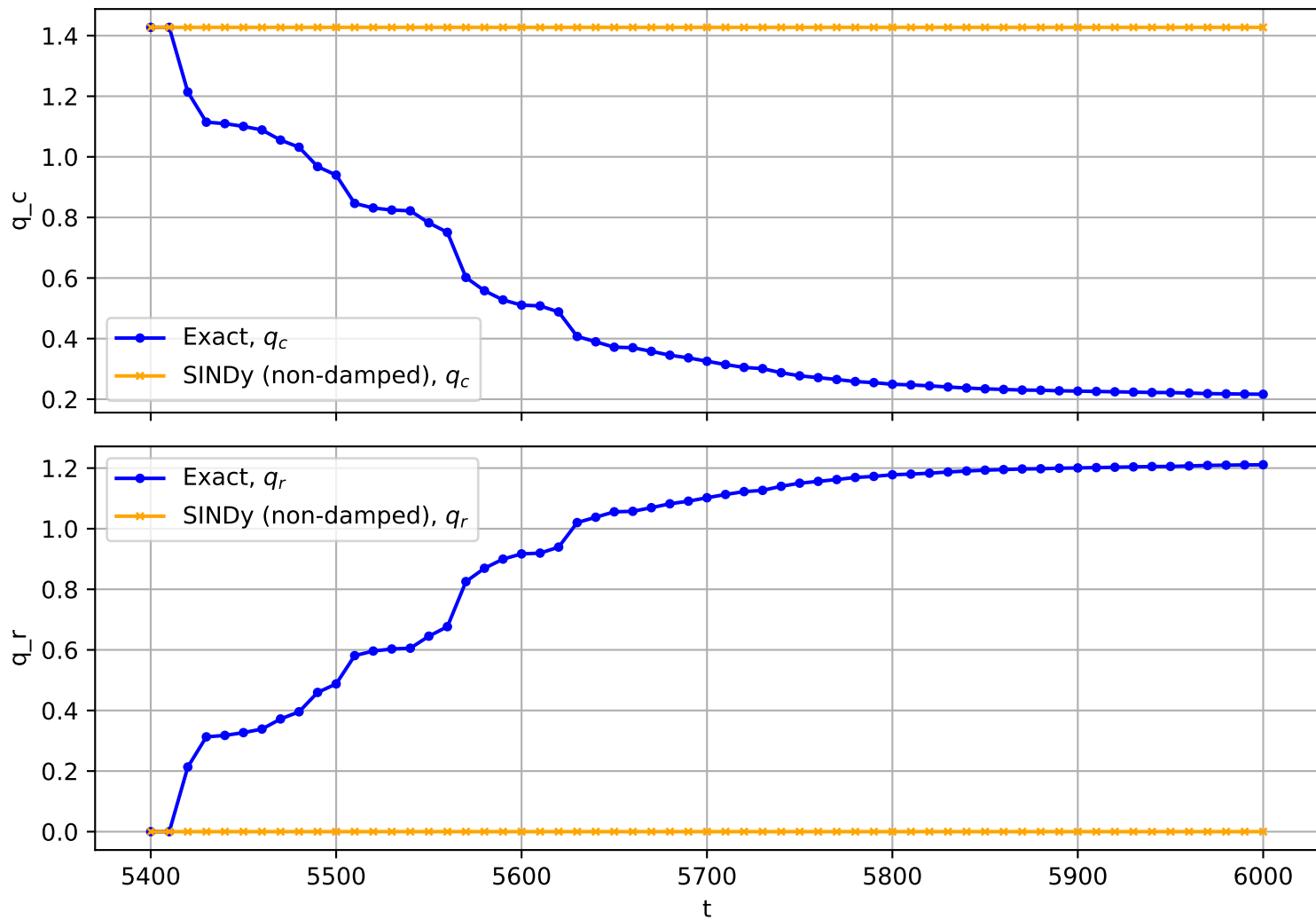
Trajectory No. 1731
