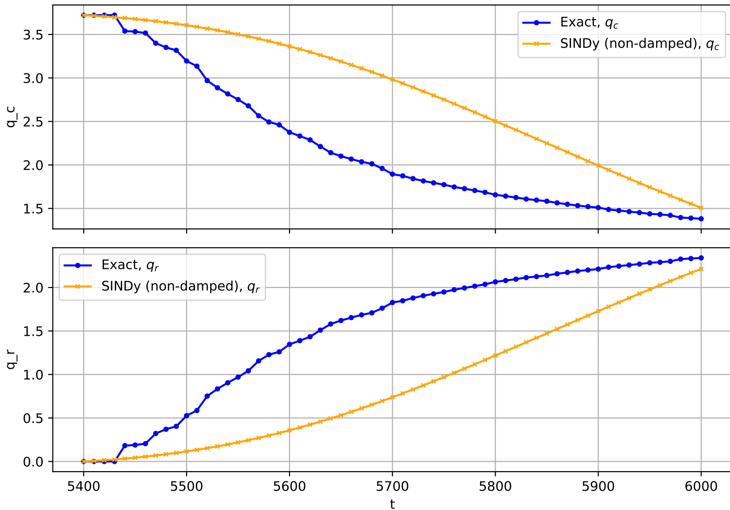
Trajectory No. 1739
