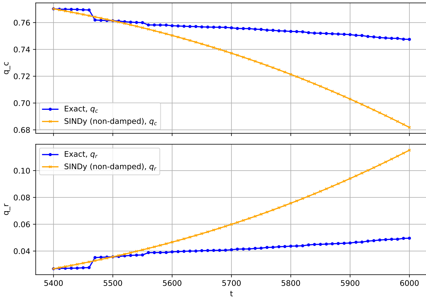
Trajectory No. 1746
