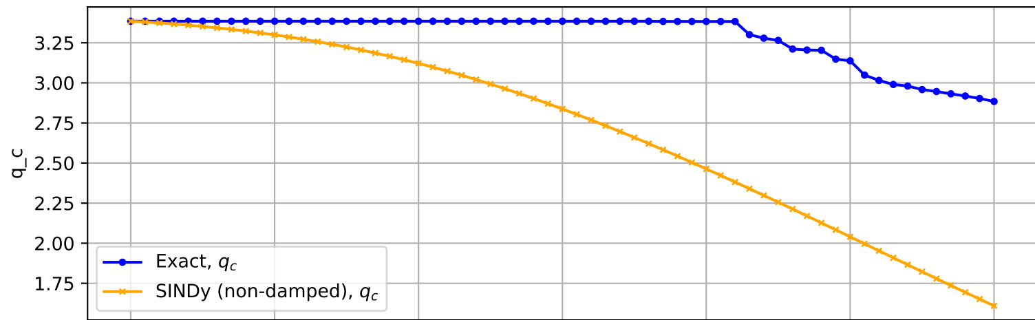
Trajectory No. 1762
