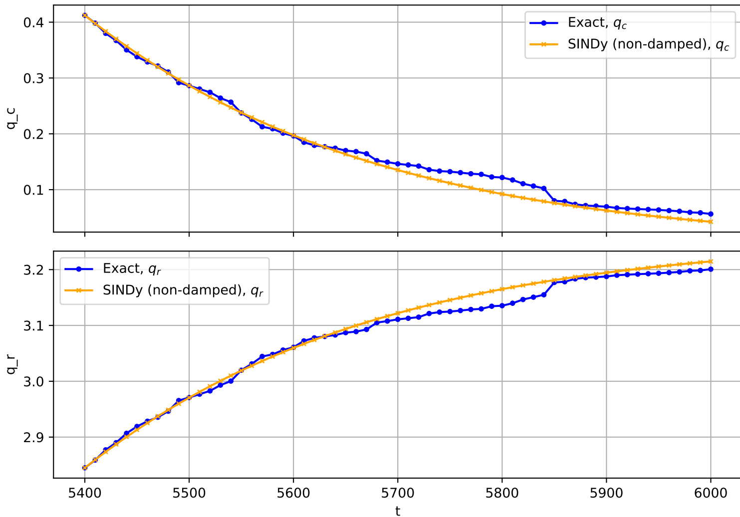
Trajectory No. 1801
