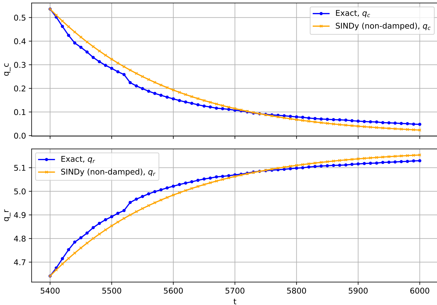
Trajectory No. 1824
