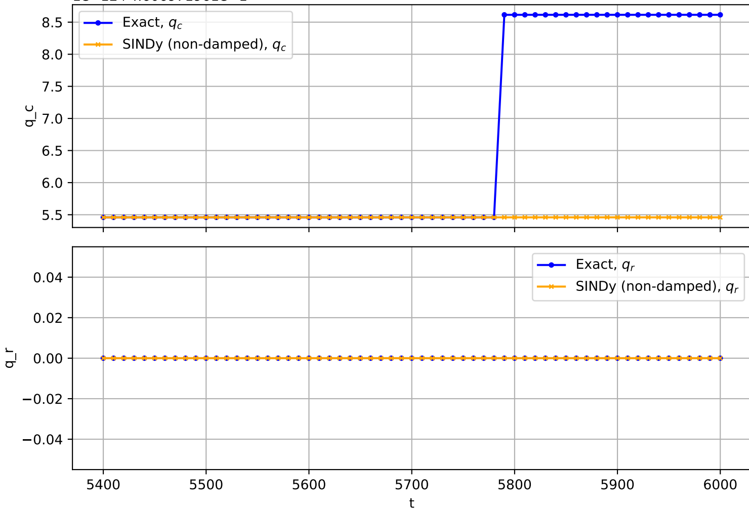
Trajectory No. 1846
