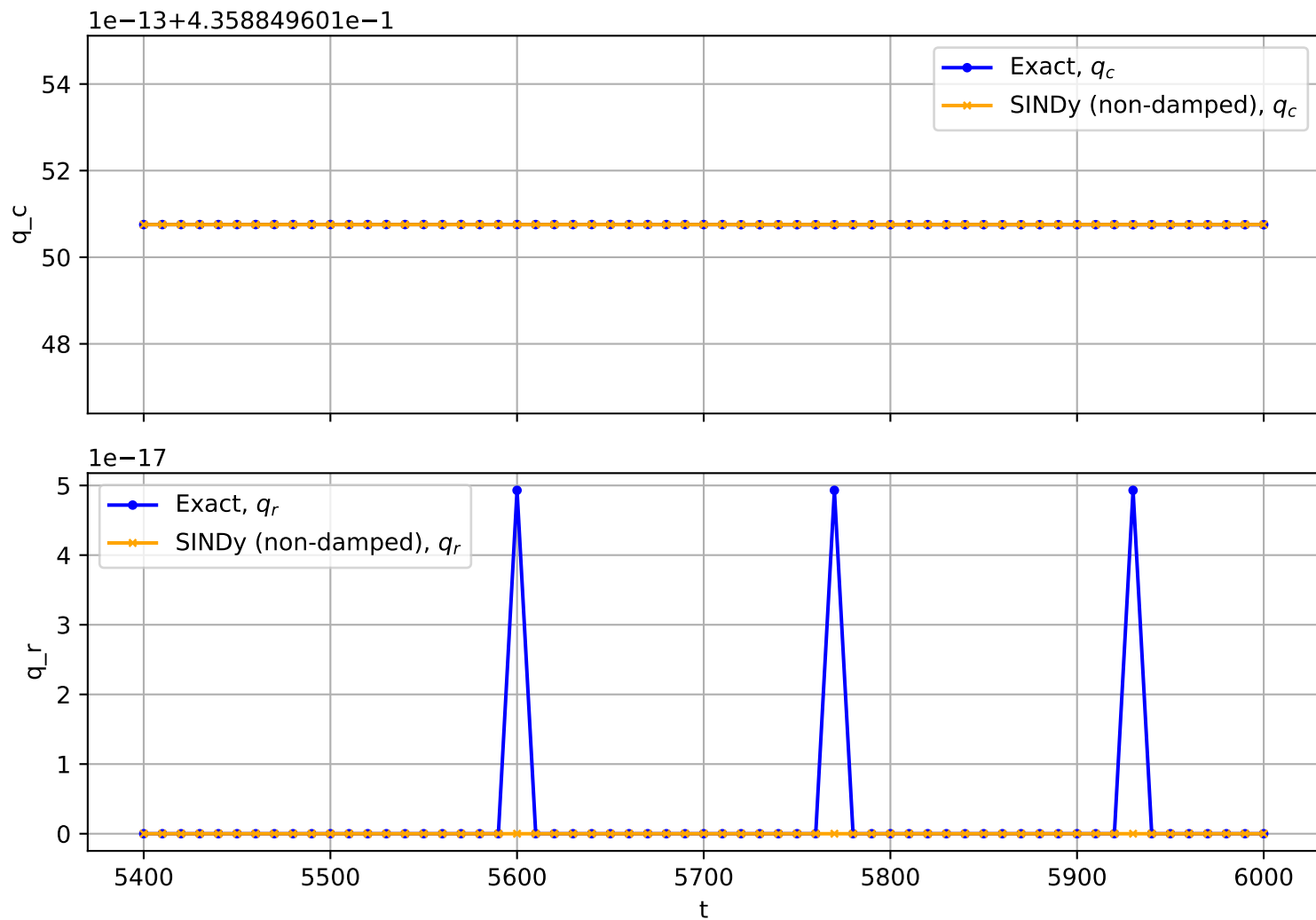
Trajectory No. 1859
