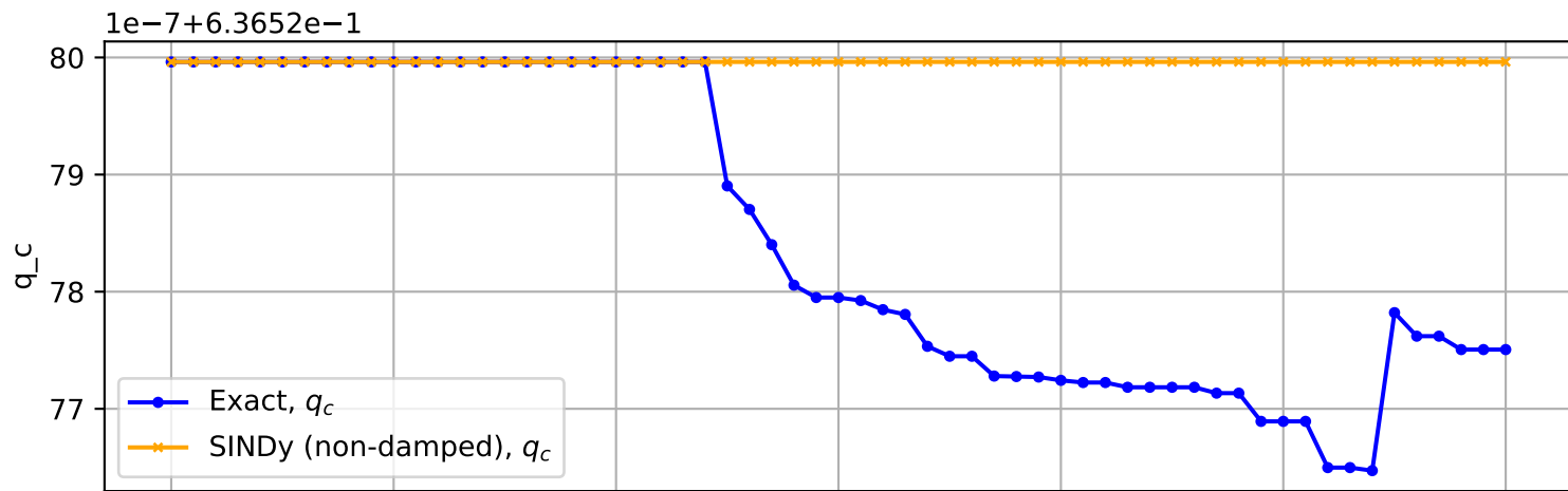
Trajectory No. 1877
