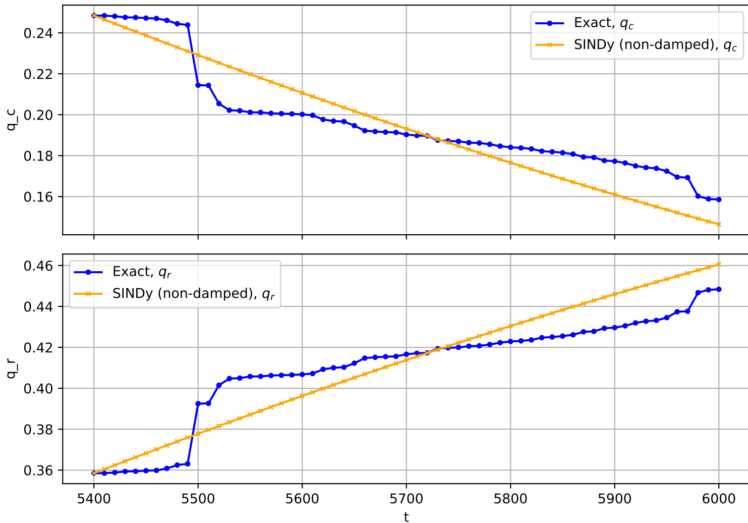
Trajectory No. 188
