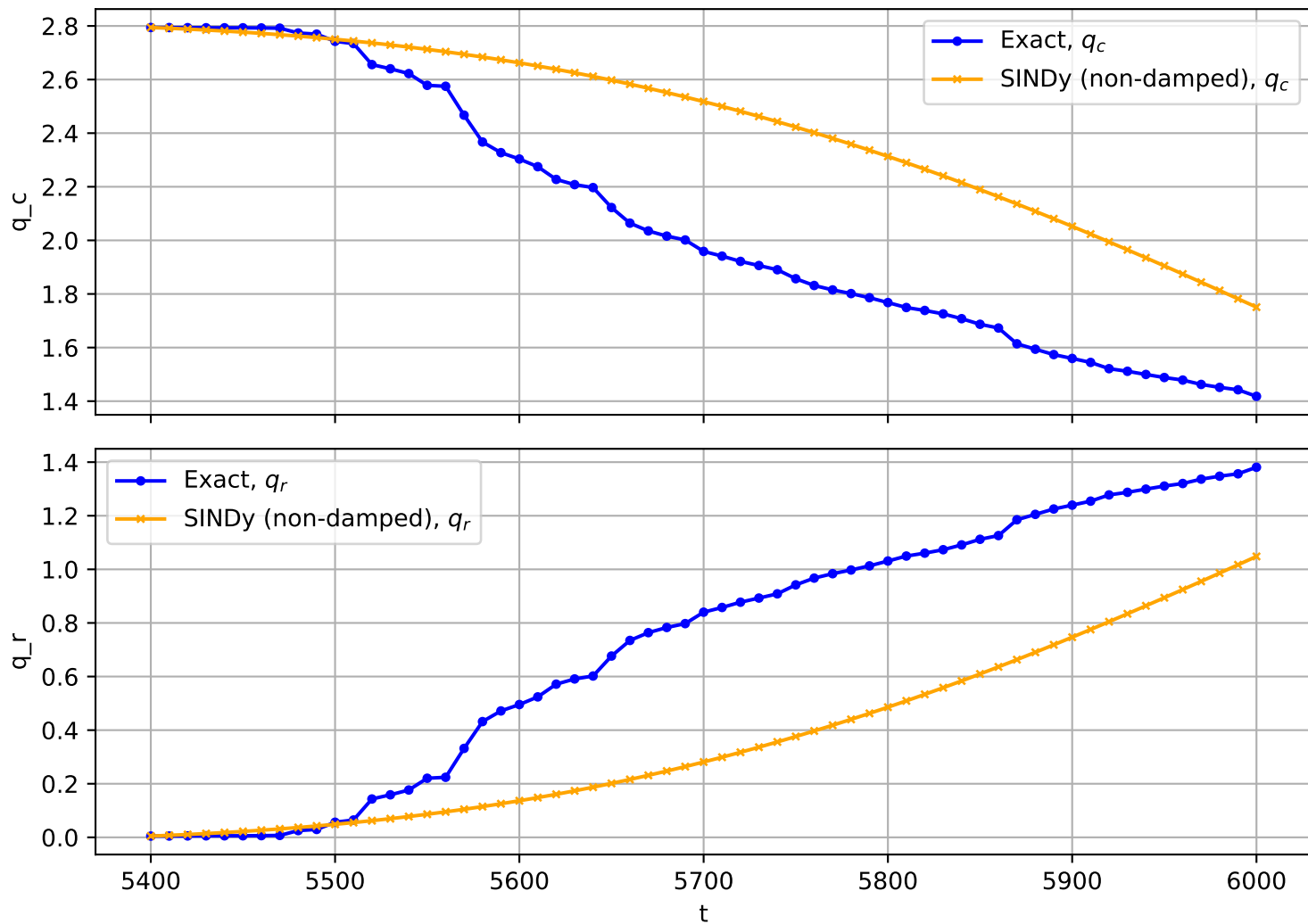
Trajectory No. 1896
