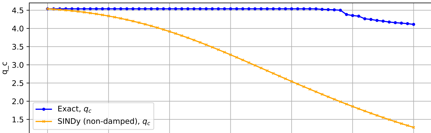
Trajectory No. 1899
