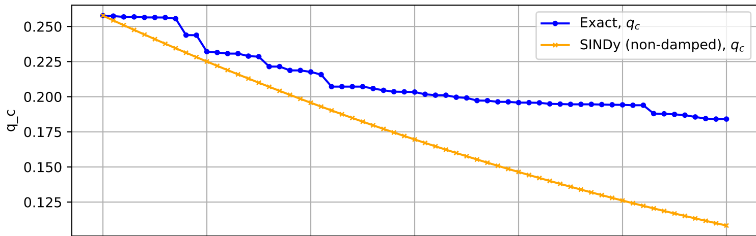
Trajectory No. 1909
