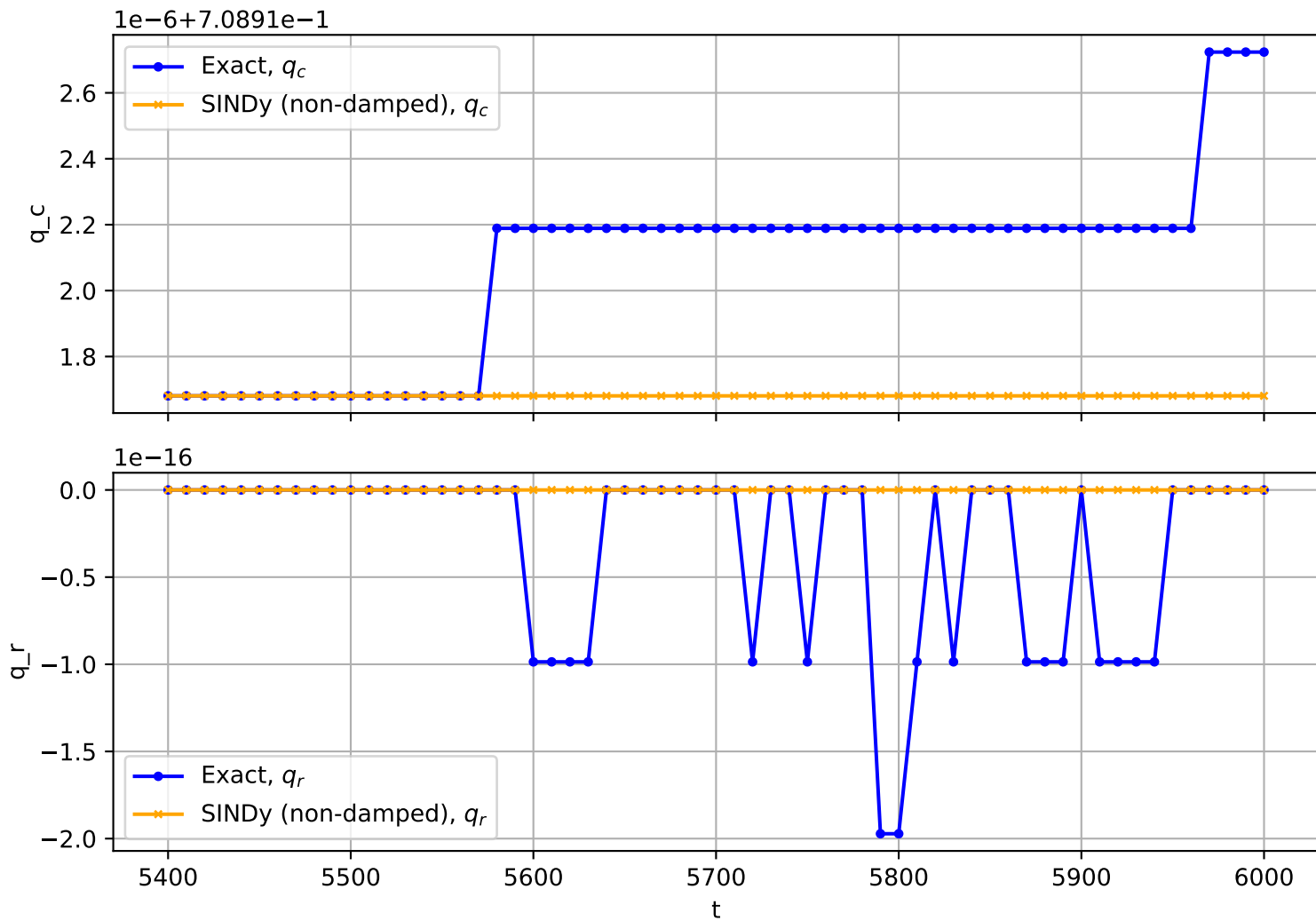
Trajectory No. 1915
