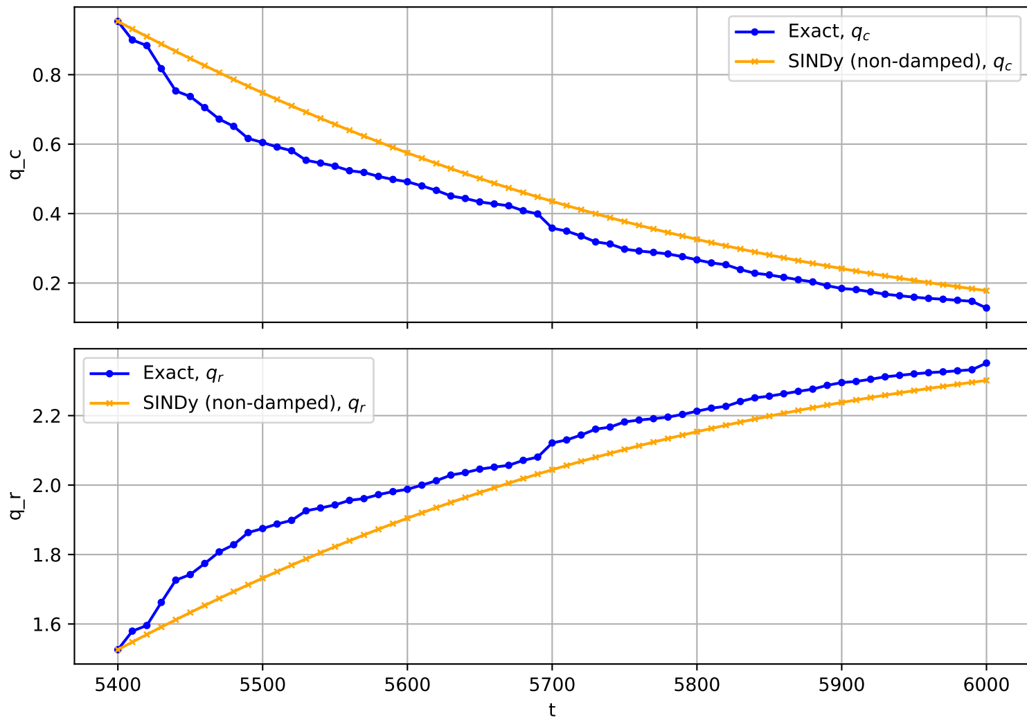
Trajectory No. 1929
