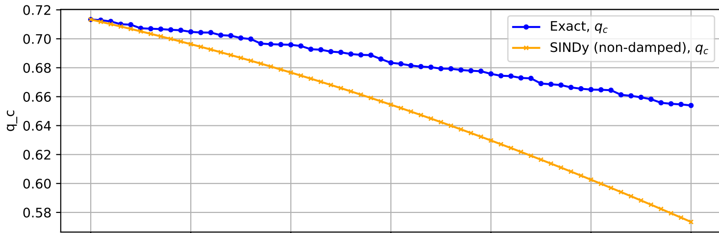
Trajectory No. 1942
