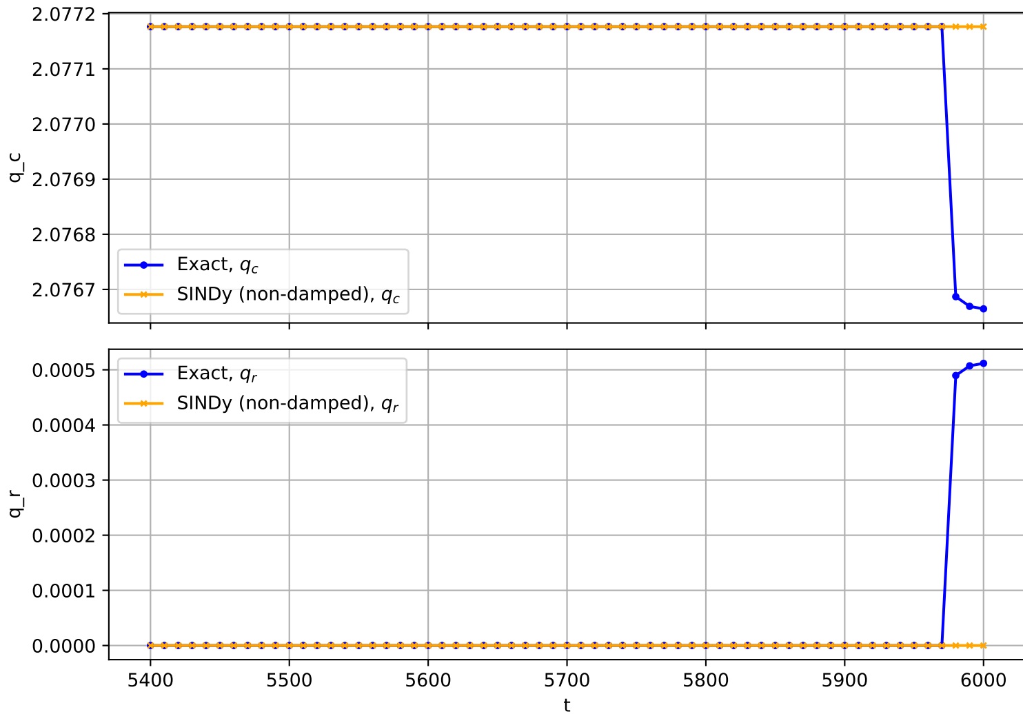
Trajectory No. 1961
