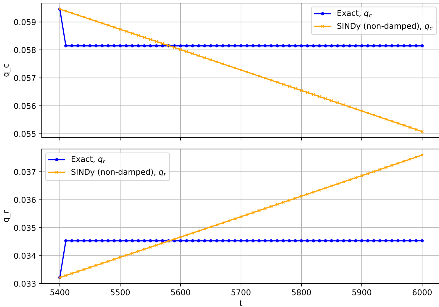
Trajectory No. 1968
