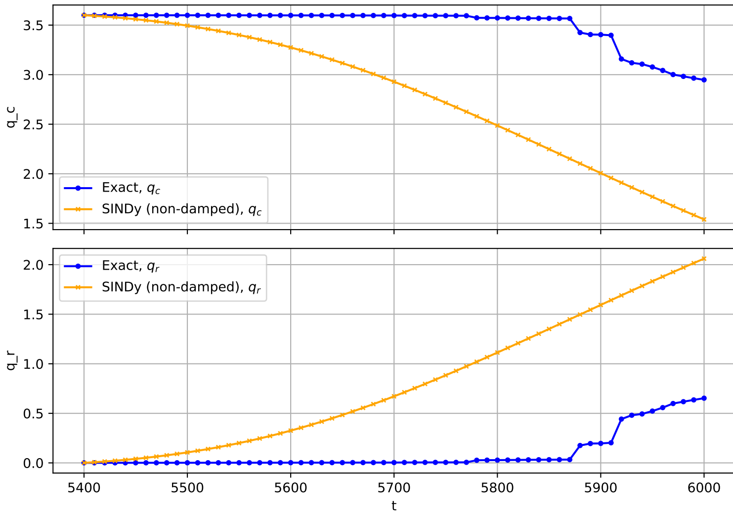
Trajectory No. 21
