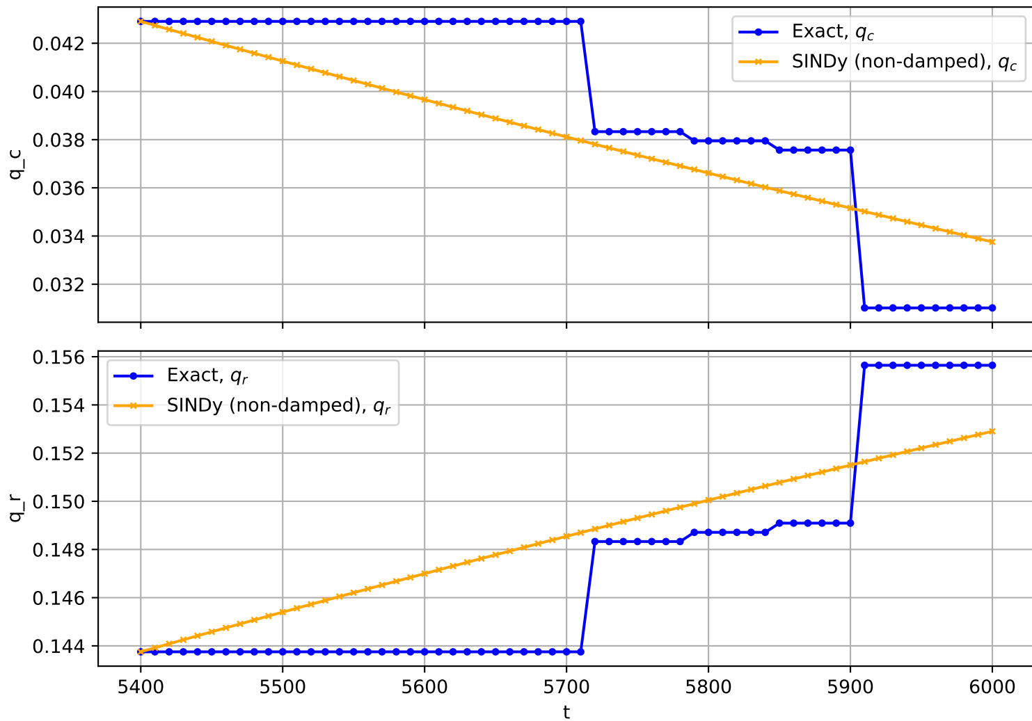
Trajectory No. 210
