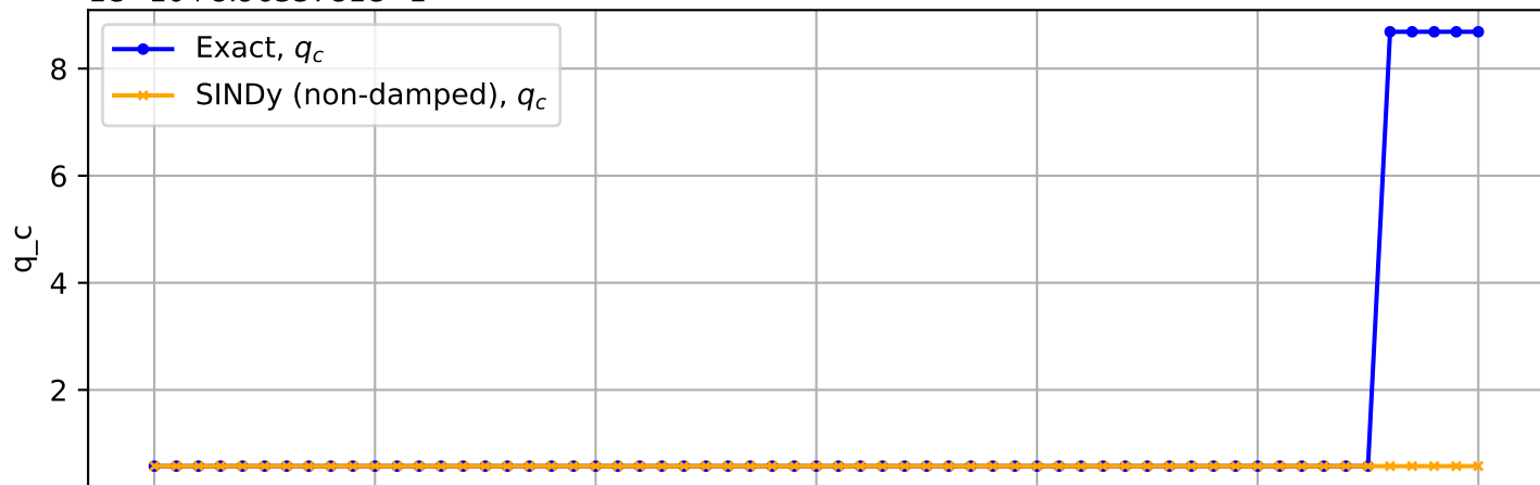
Trajectory No. 220
