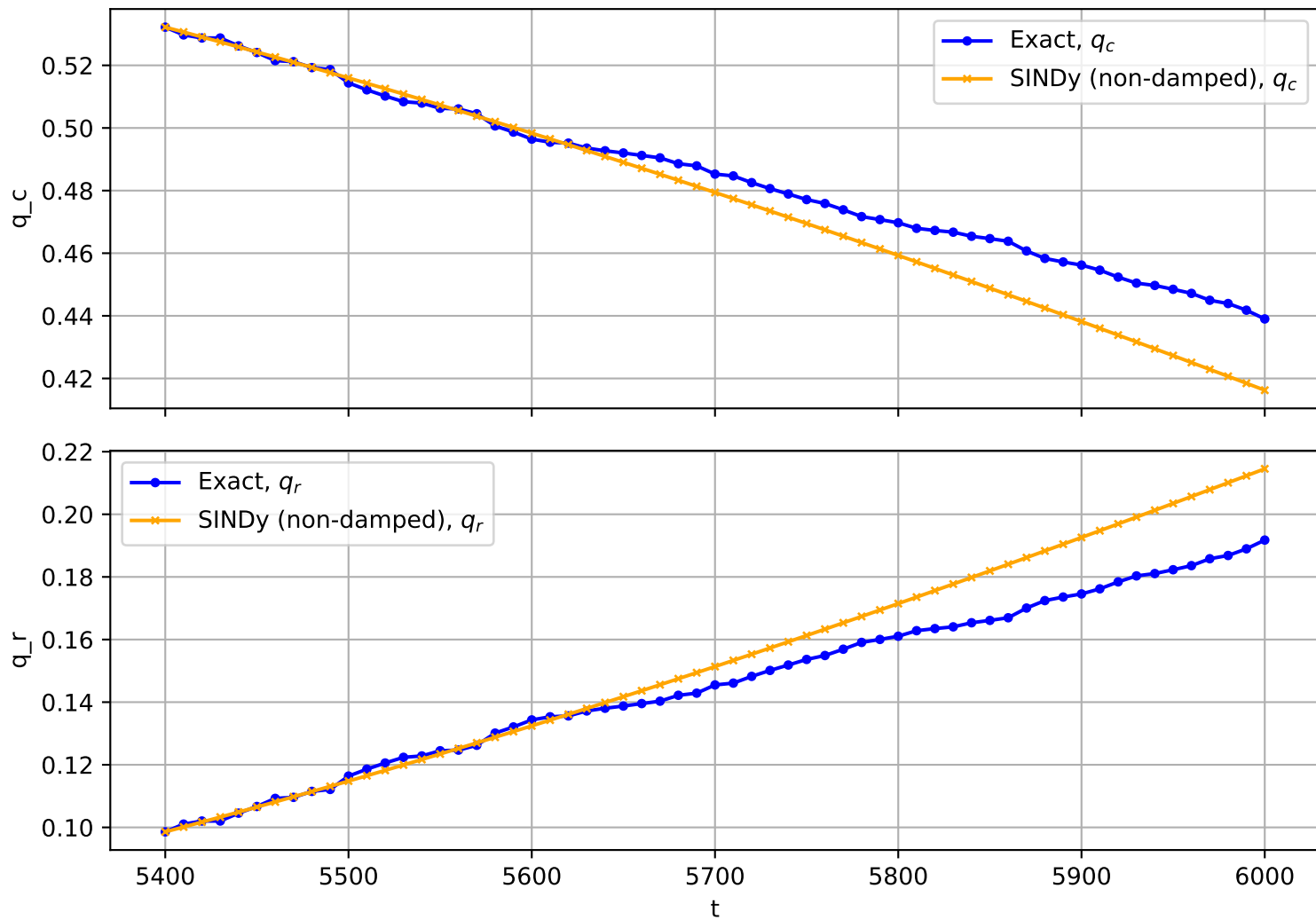
Trajectory No. 23
