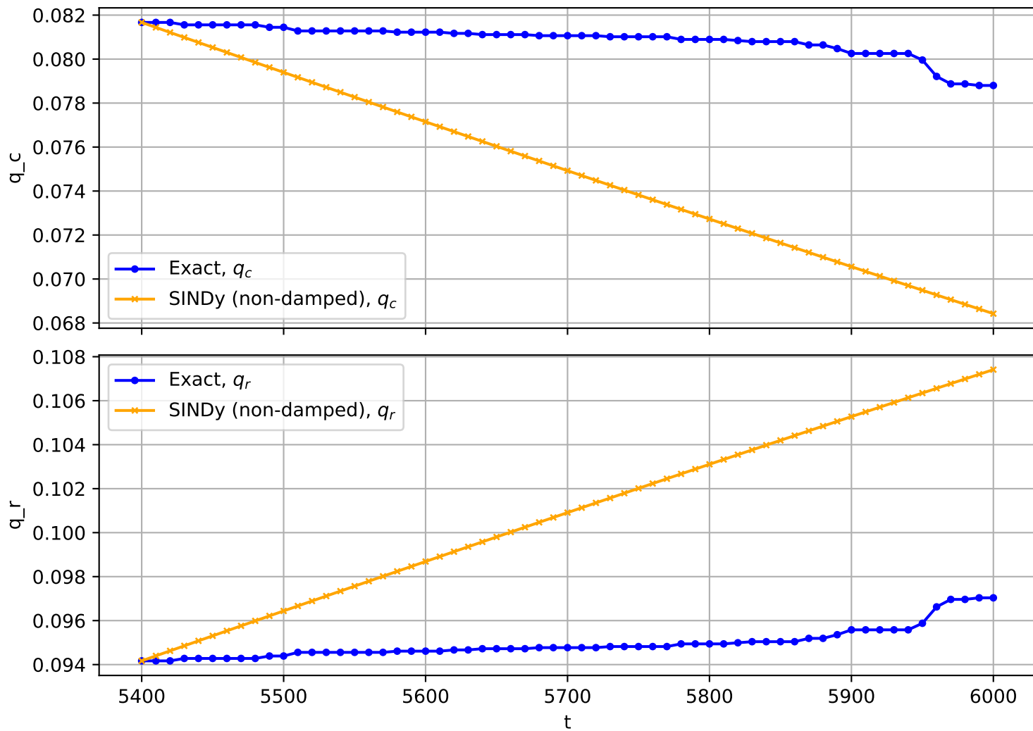
Trajectory No. 2329
