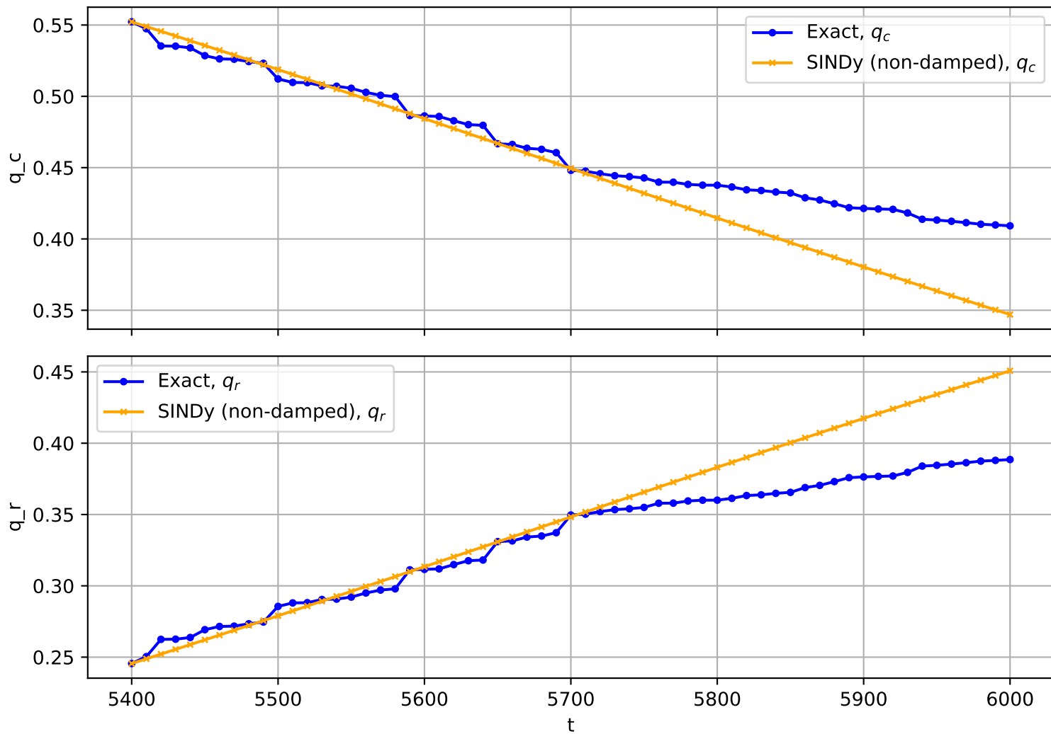
Trajectory No. 2350
