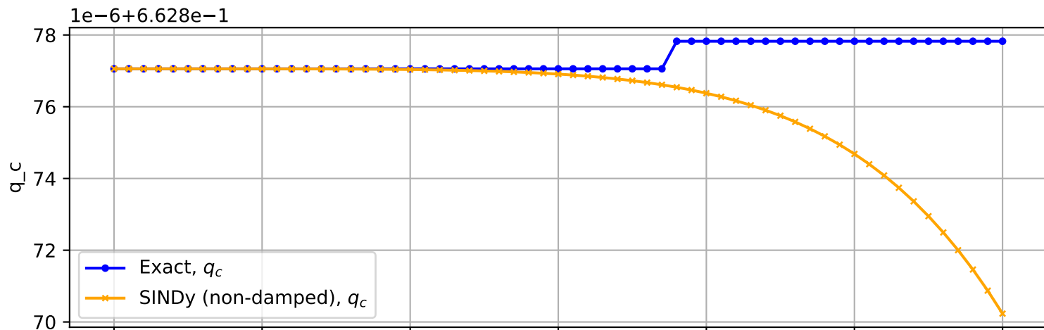
Trajectory No. 2428
