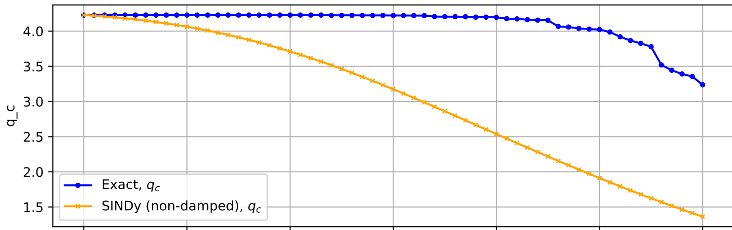
Trajectory No. 2505
