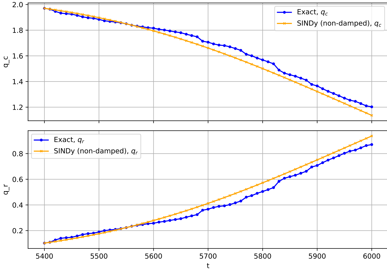
Trajectory No. 251
