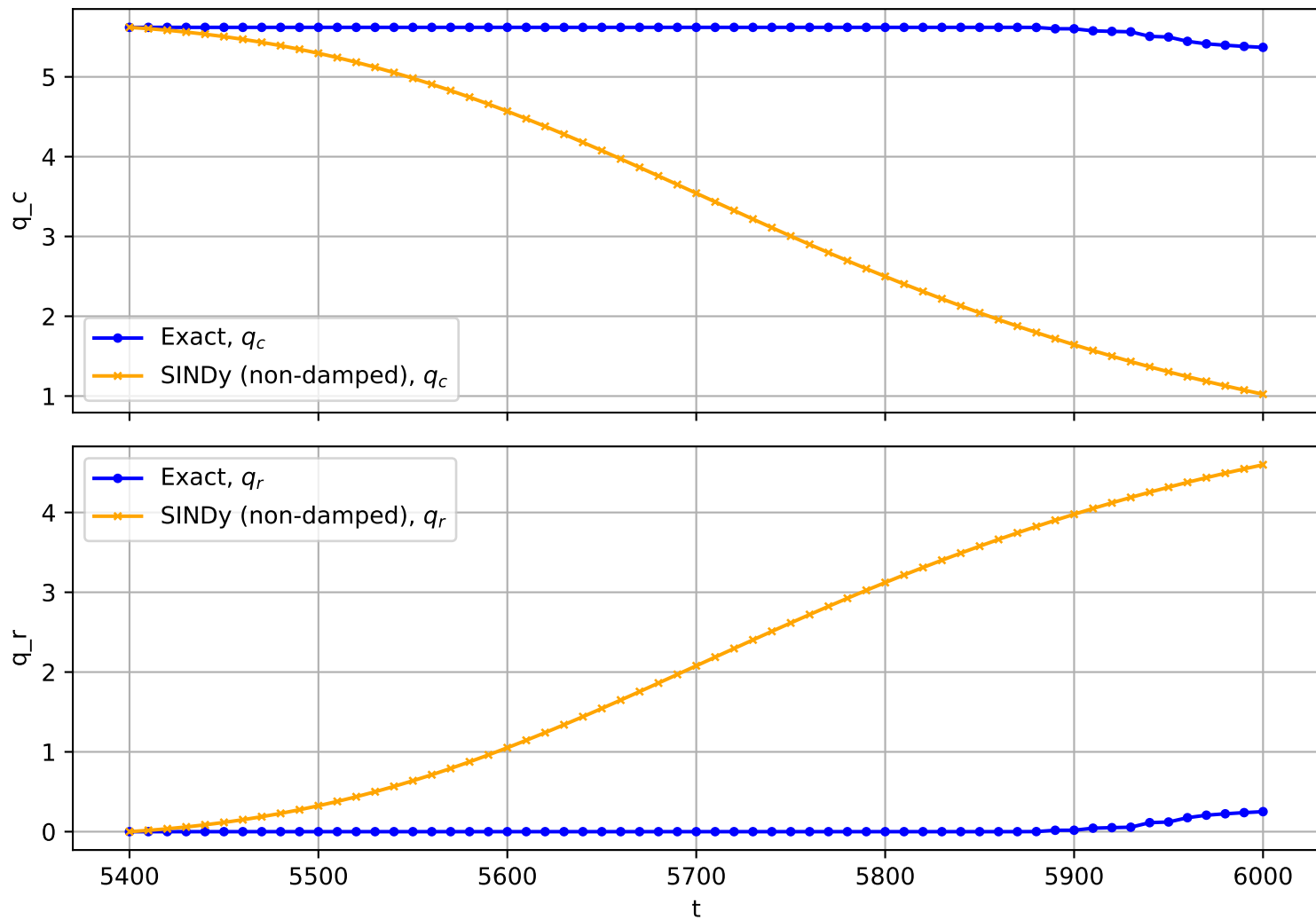
Trajectory No. 2522
