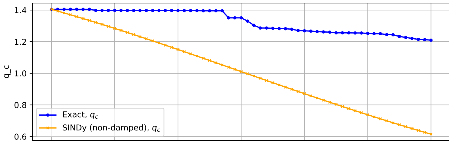
Trajectory No. 2552
