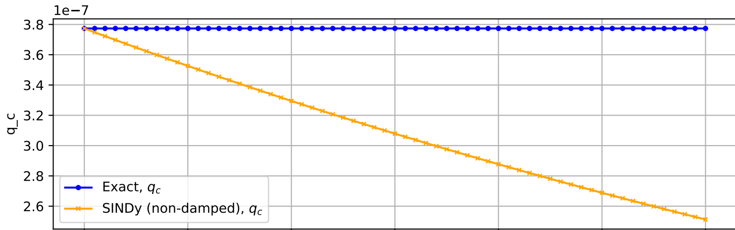
Trajectory No. 2554
