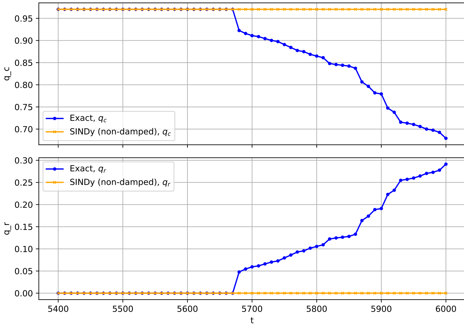
Trajectory No. 2560
