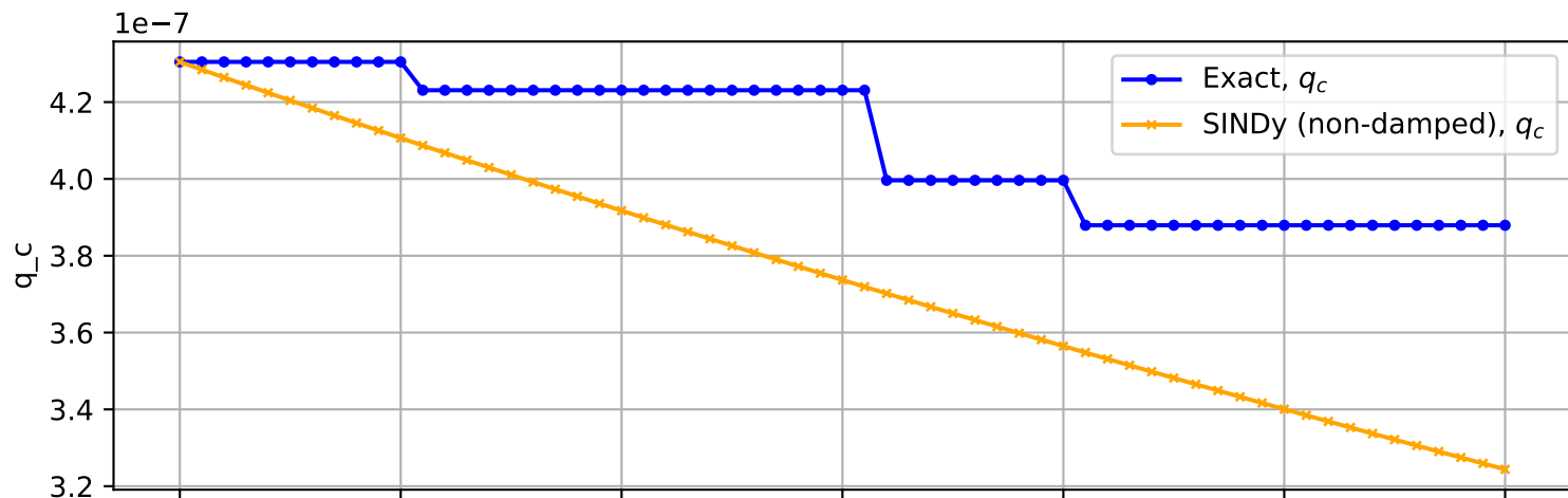
Trajectory No. 2561
