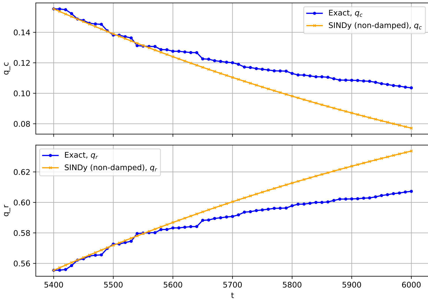
Trajectory No. 2582
