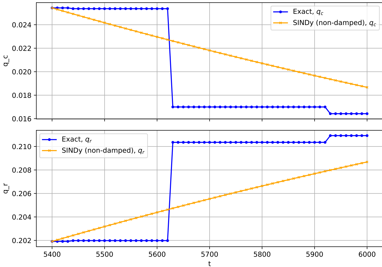
Trajectory No. 2584
