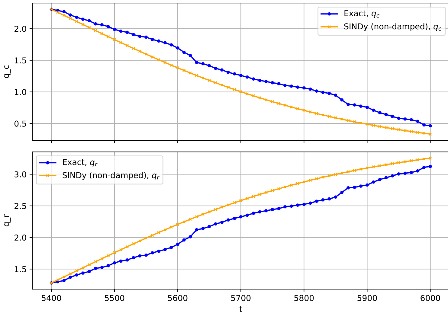
Trajectory No. 2605
