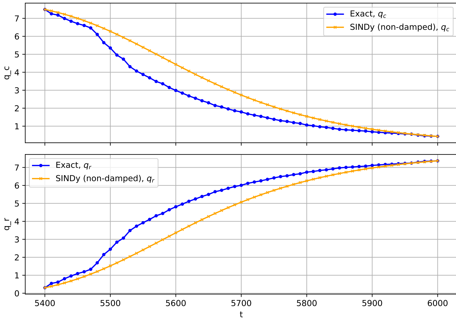
Trajectory No. 2606
