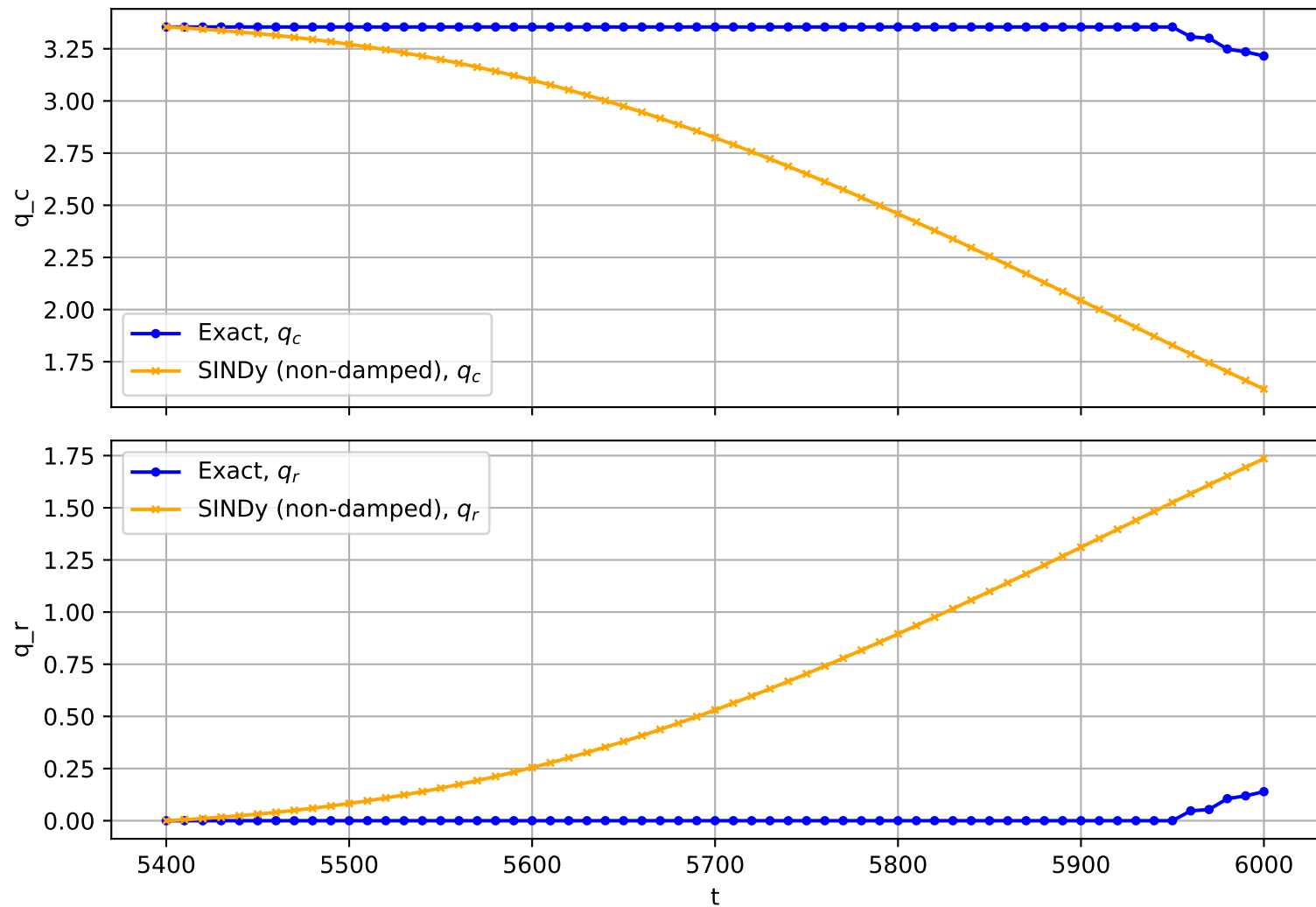
Trajectory No. 2632
