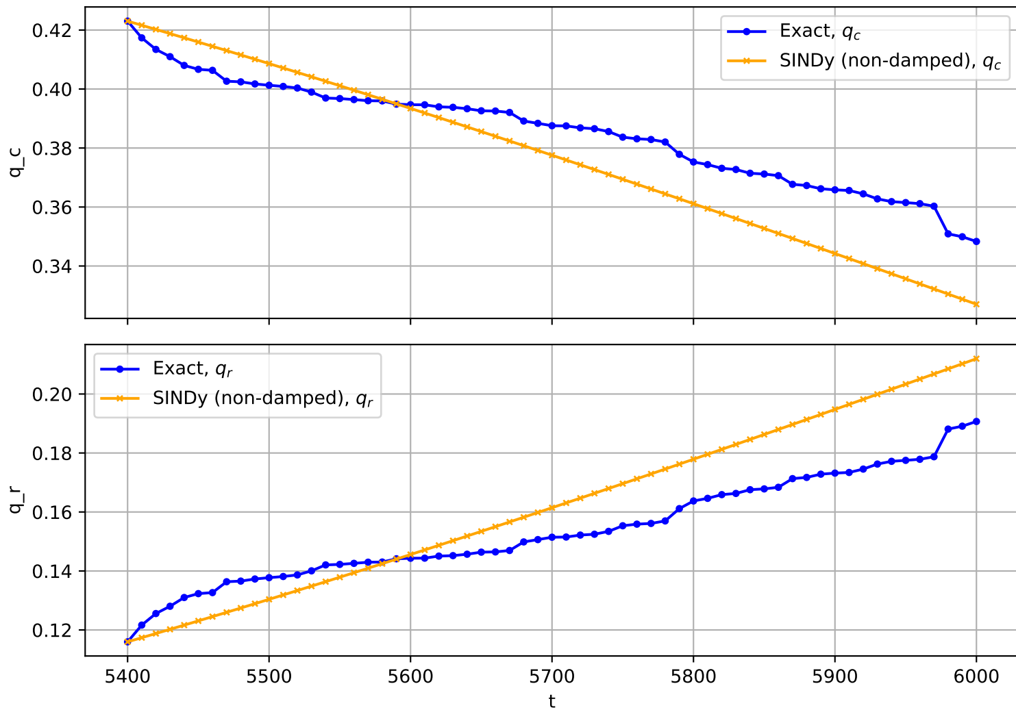
Trajectory No. 2662
