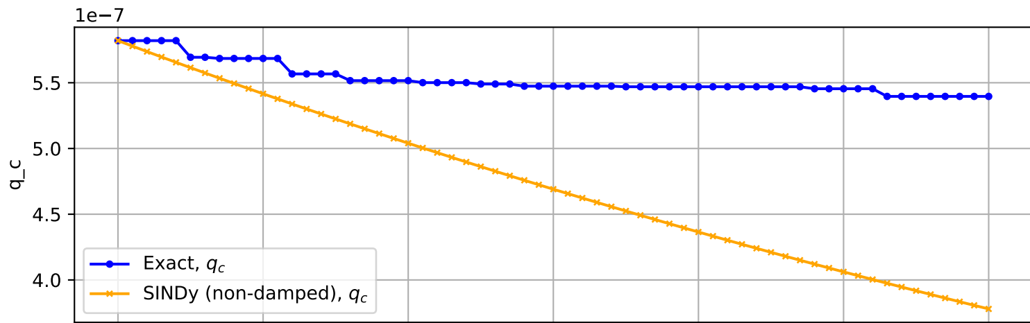
Trajectory No. 2675
