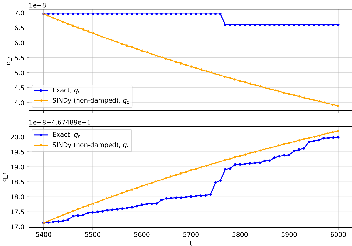
Trajectory No. 2693
