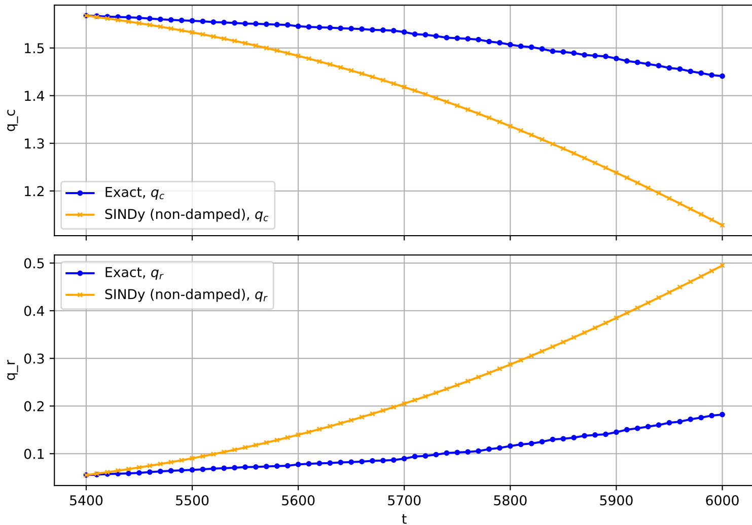
Trajectory No. 2699
